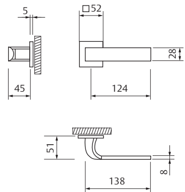
Dimensions (mm)
