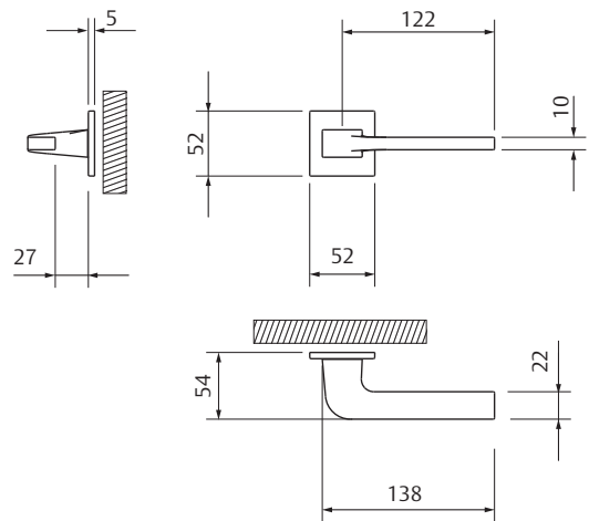
Dimensions (mm)
