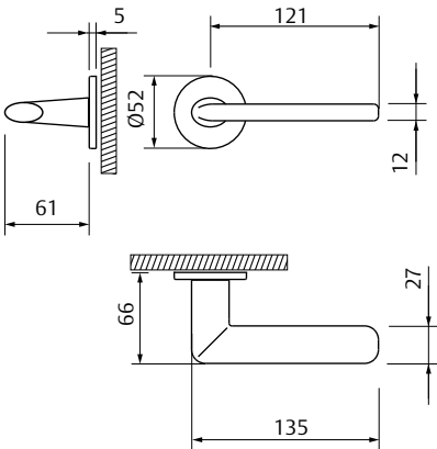
Dimensions (mm)
