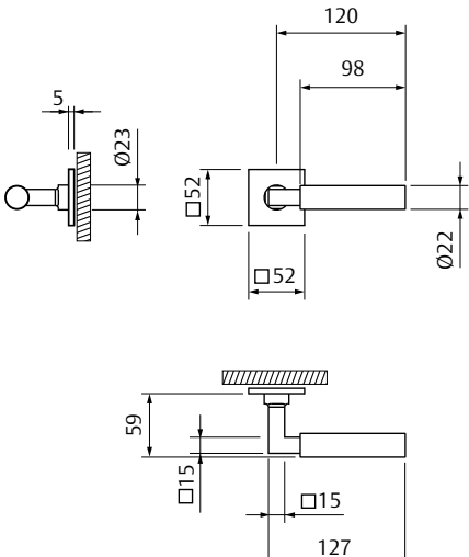
Dimensions (mm)
